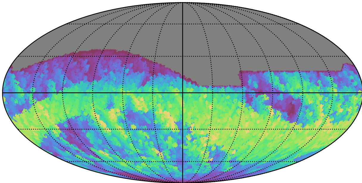
ddf_loaded_half_fl2_v3.4_10yrs All sky r band: Max normairmass
