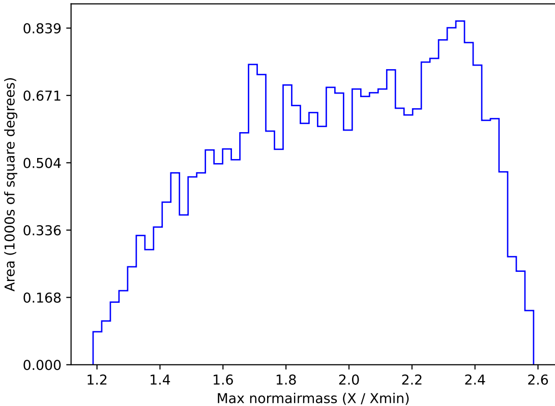
ddf_loaded_half_fl2_v3.4_10yrs All sky r band: Max normairmass
