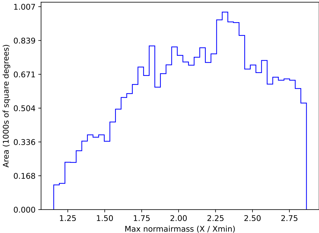
ddf_loaded_half_fl2_v3.4_10yrs All sky i band: Max normairmass
