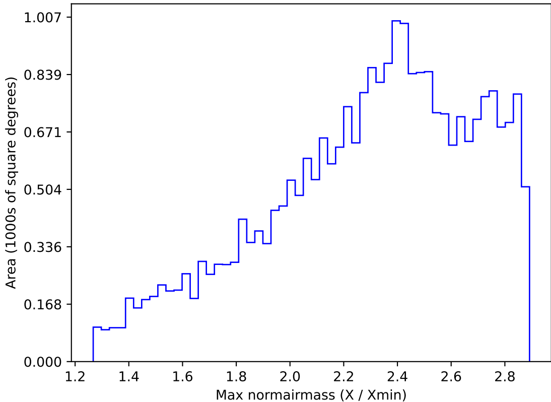
ddf_loaded_half_fl2_v3.4_10yrs All sky all bands: Max normairmass
