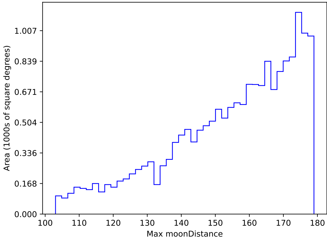
ddf_loaded_half_fl2_v3.4_10yrs WFD z band: Max moonDistance
