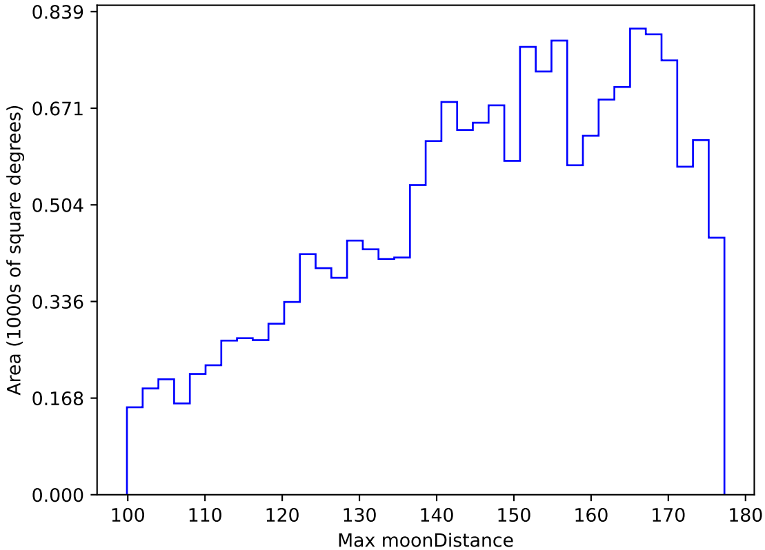
ddf_loaded_half_fl2_v3.4_10yrs WFD y band: Max moonDistance
