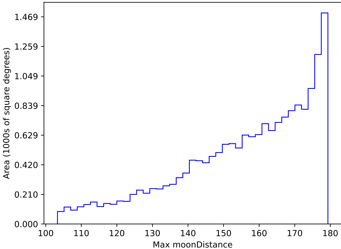
ddf_loaded_half_fl2_v3.4_10yrs WFD r band: Max moonDistance
