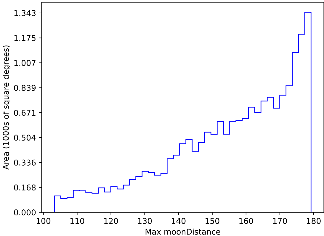
ddf_loaded_half_fl2_v3.4_10yrs WFD i band: Max moonDistance
