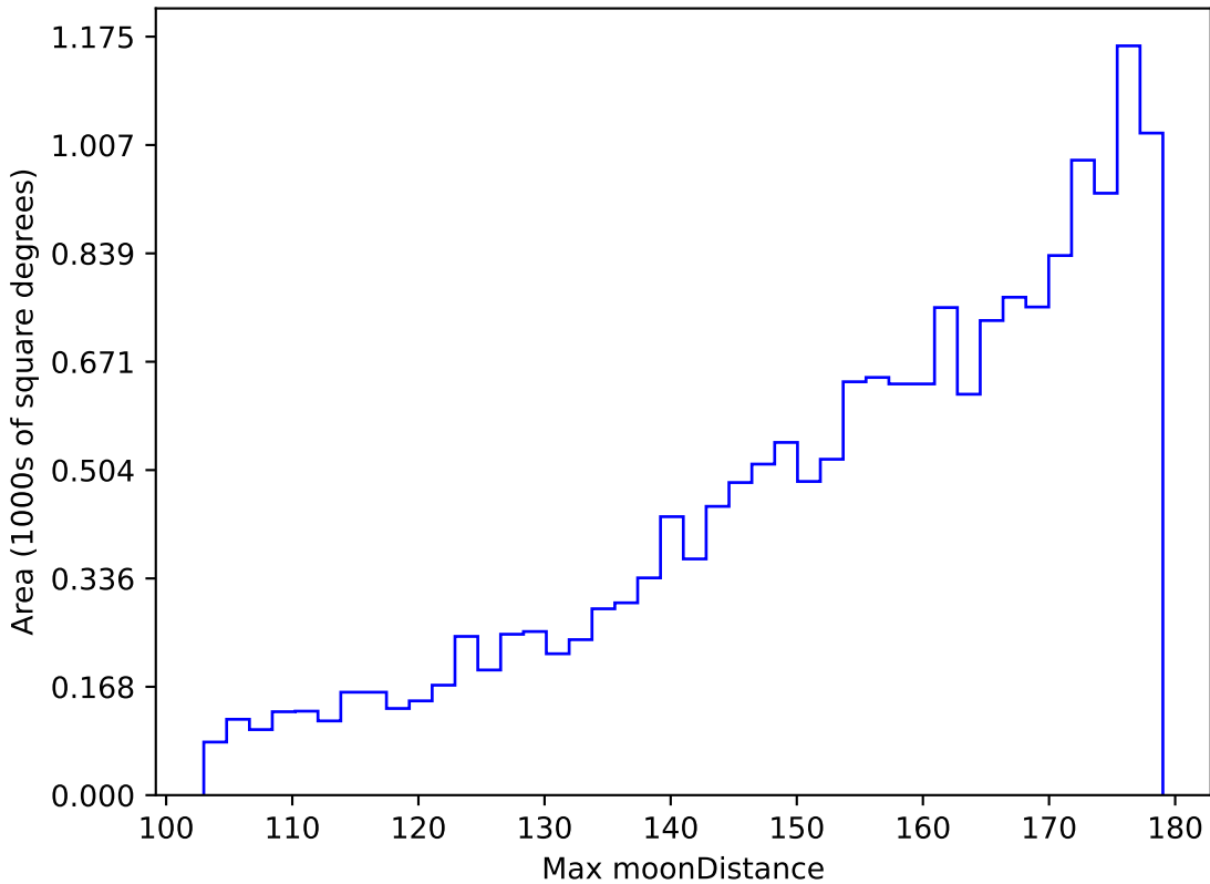
ddf_loaded_half_fl2_v3.4_10yrs WFD g band: Max moonDistance
