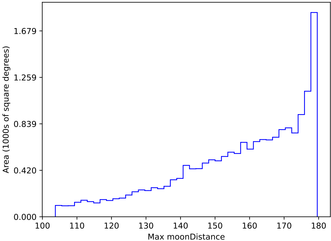
ddf_loaded_half_fl2_v3.4_10yrs WFD all bands: Max moonDistance
