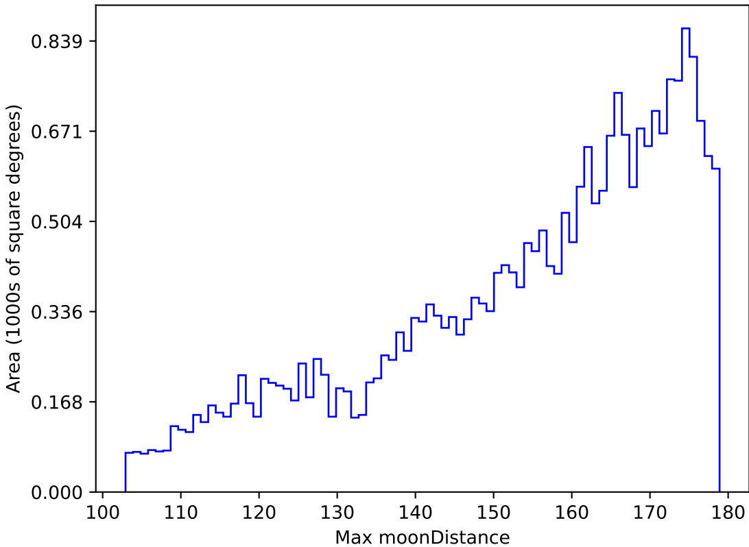
ddf_loaded_half_fl2_v3.4_10yrs All sky z band: Max moonDistance
