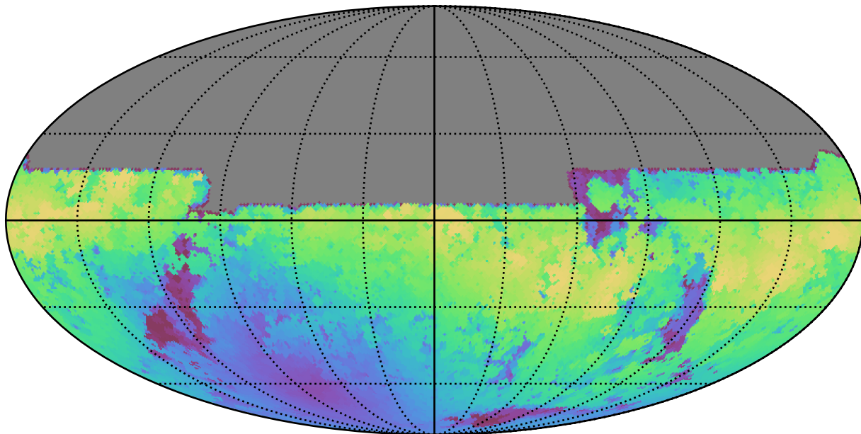
ddf_loaded_half_fl2_v3.4_10yrs All sky y band: Max moonDistance
