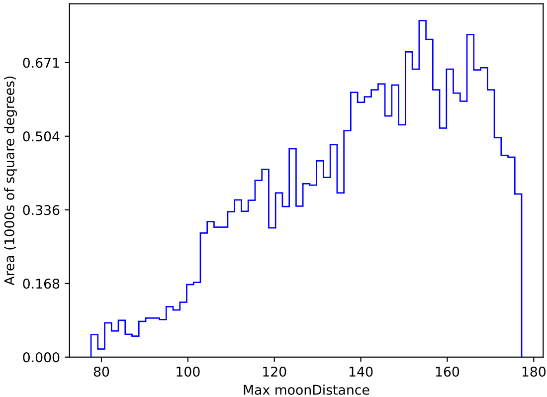
ddf_loaded_half_fl2_v3.4_10yrs All sky y band: Max moonDistance
