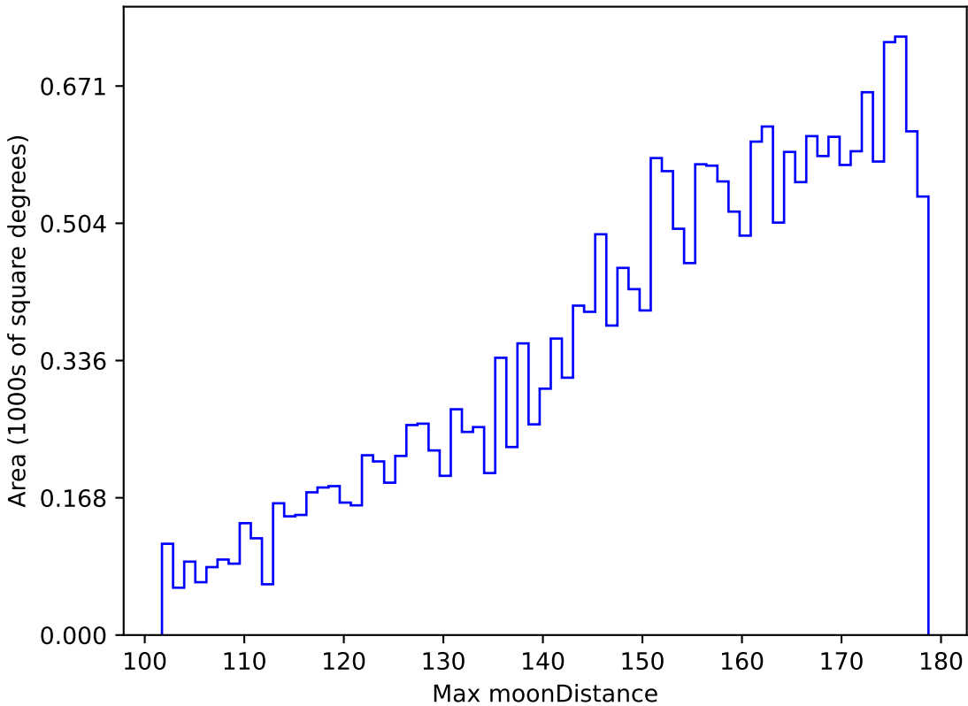
ddf_loaded_half_fl2_v3.4_10yrs All sky u band: Max moonDistance
