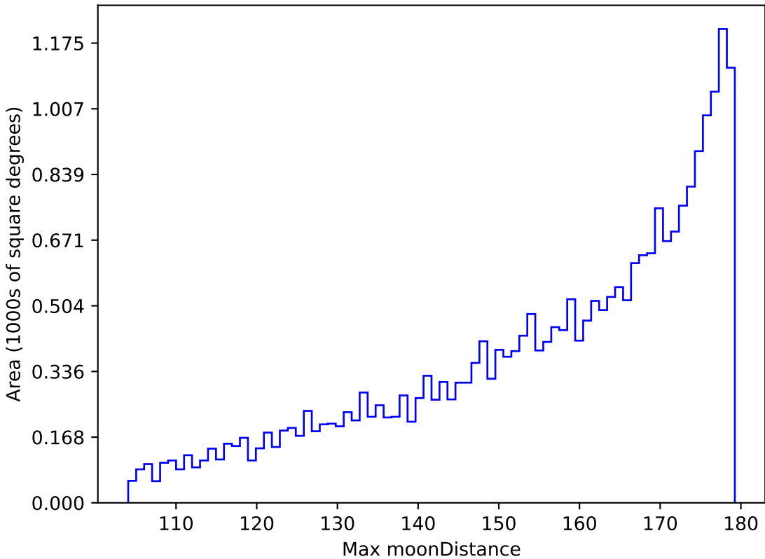
ddf_loaded_half_fl2_v3.4_10yrs All sky r band: Max moonDistance
