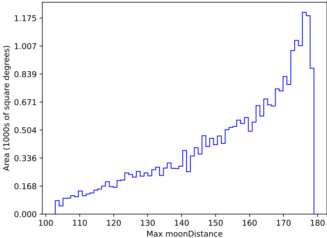
ddf_loaded_half_fl2_v3.4_10yrs All sky g band: Max moonDistance
