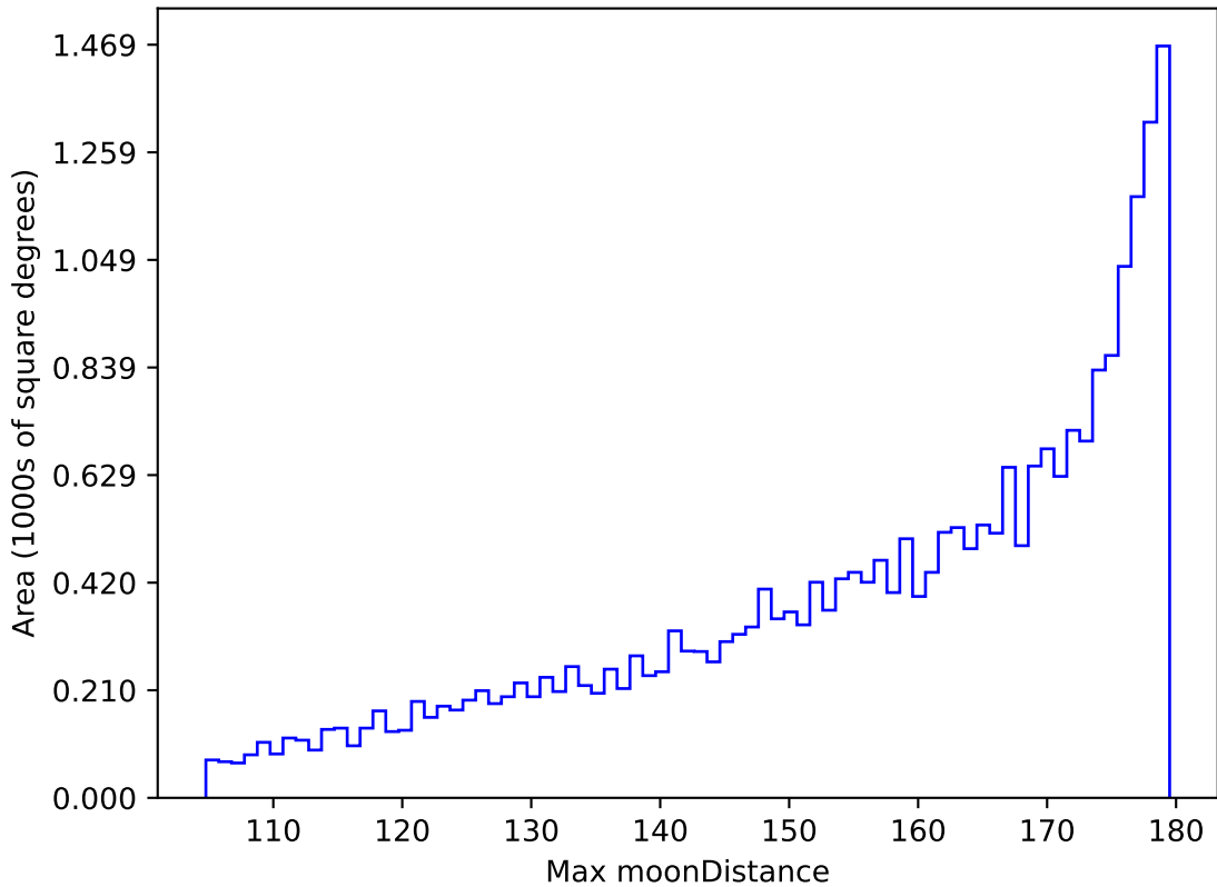
ddf_loaded_half_fl2_v3.4_10yrs All sky all bands: Max moonDistance
