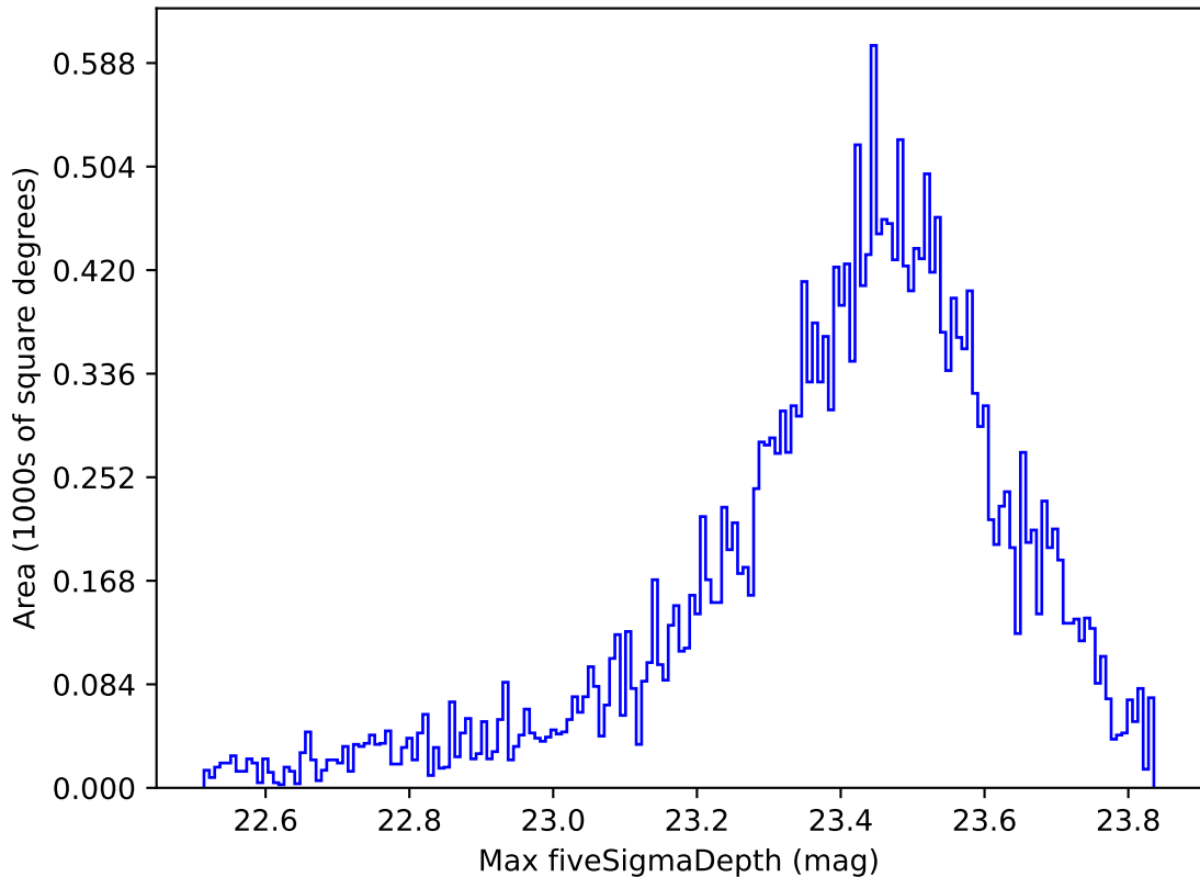
ddf_loaded_half_fl2_v3.4_10yrs Yr 1 z band: Max fiveSigmaDepth
