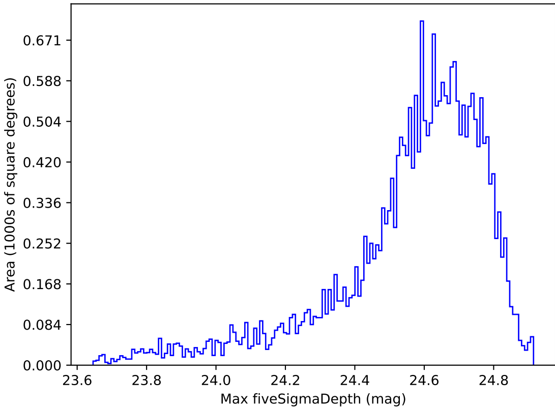
ddf_loaded_half_fl2_v3.4_10yrs Yr 1 r band: Max fiveSigmaDepth
