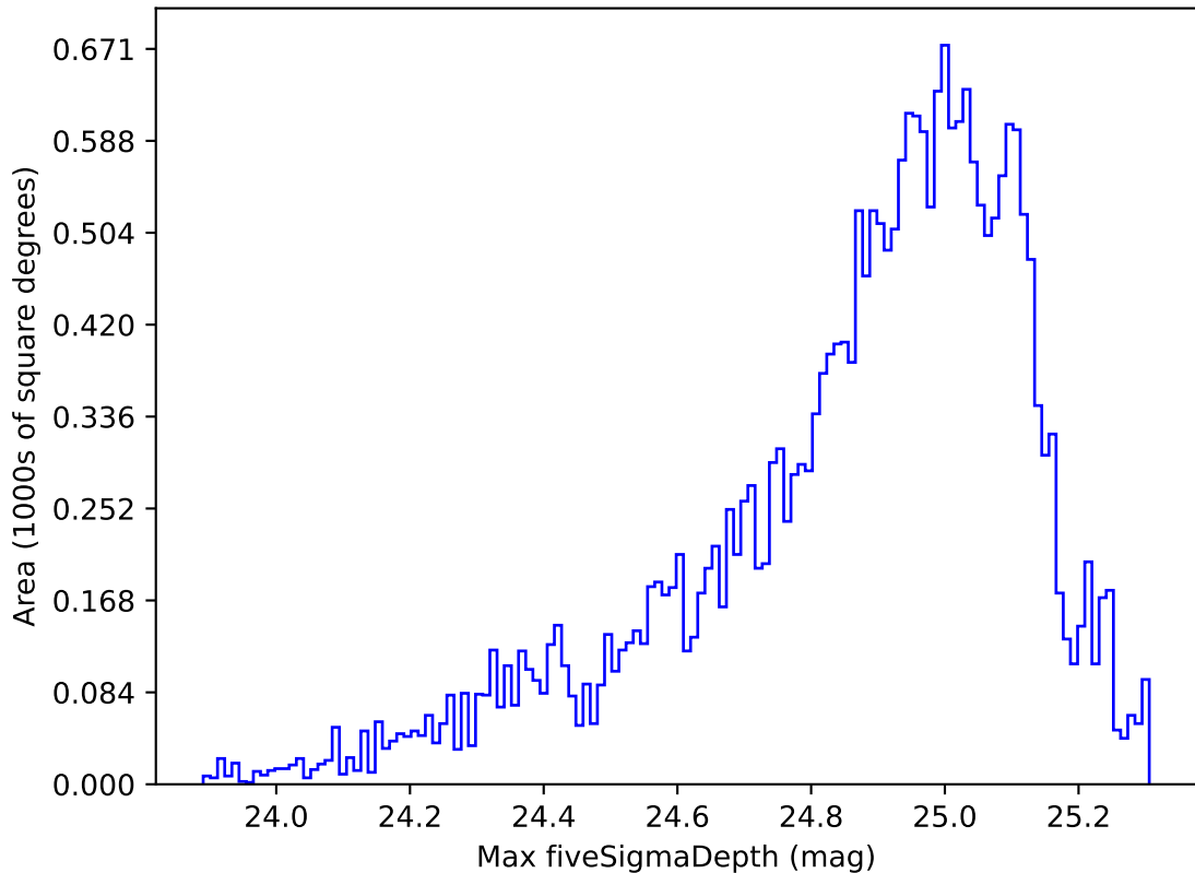
ddf_loaded_half_fl2_v3.4_10yrs Yr 1 g band: Max fiveSigmaDepth
