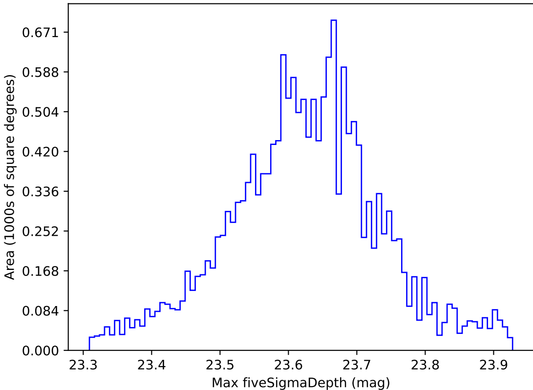
ddf_loaded_half_fl2_v3.4_10yrs WFD z band: Max fiveSigmaDepth
