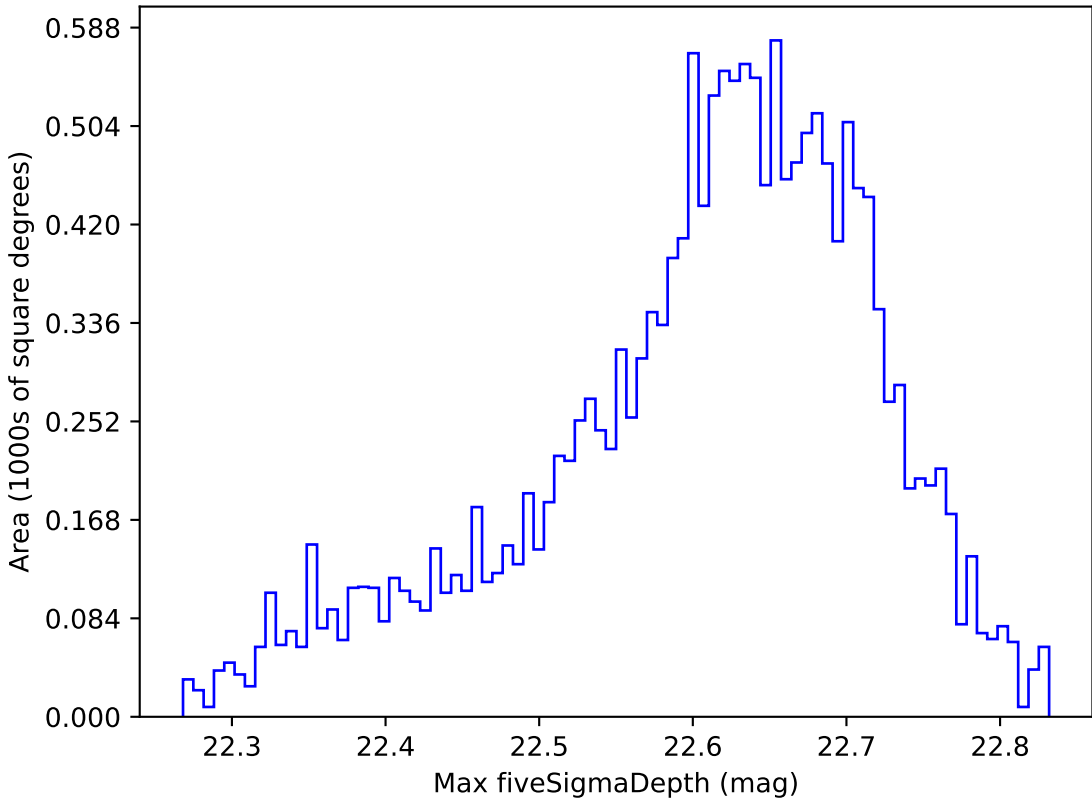
ddf_loaded_half_fl2_v3.4_10yrs WFD y band: Max fiveSigmaDepth
