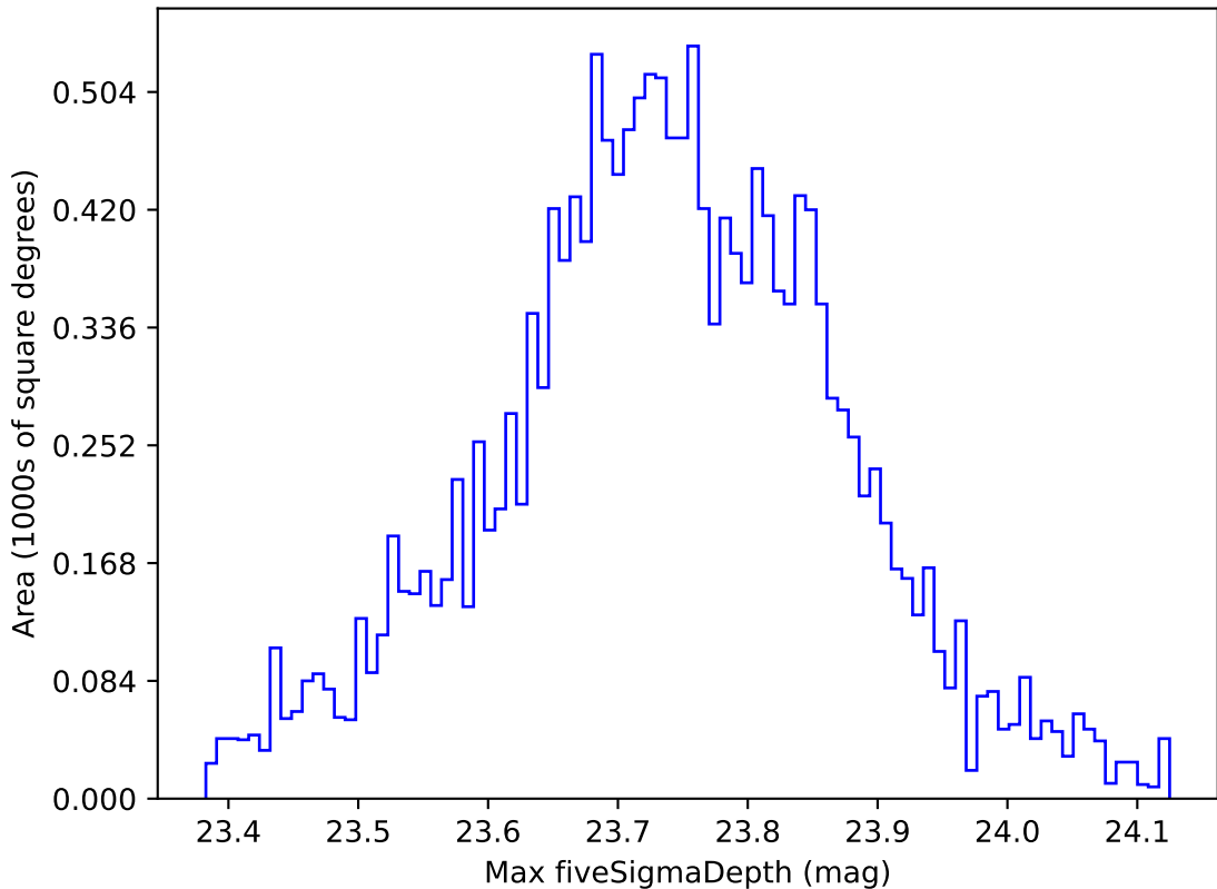
ddf_loaded_half_fl2_v3.4_10yrs WFD u band: Max fiveSigmaDepth
