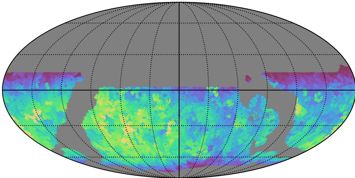
ddf_loaded_half_fl2_v3.4_10yrs WFD r band: Max fiveSigmaDepth
