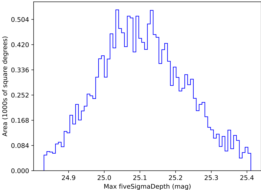
ddf_loaded_half_fl2_v3.4_10yrs WFD g band: Max fiveSigmaDepth
