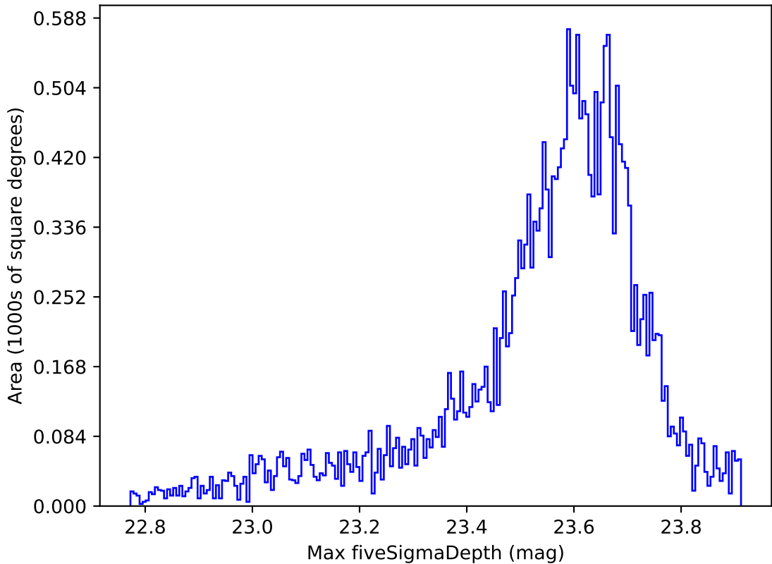
ddf_loaded_half_fl2_v3.4_10yrs All sky z band: Max fiveSigmaDepth
