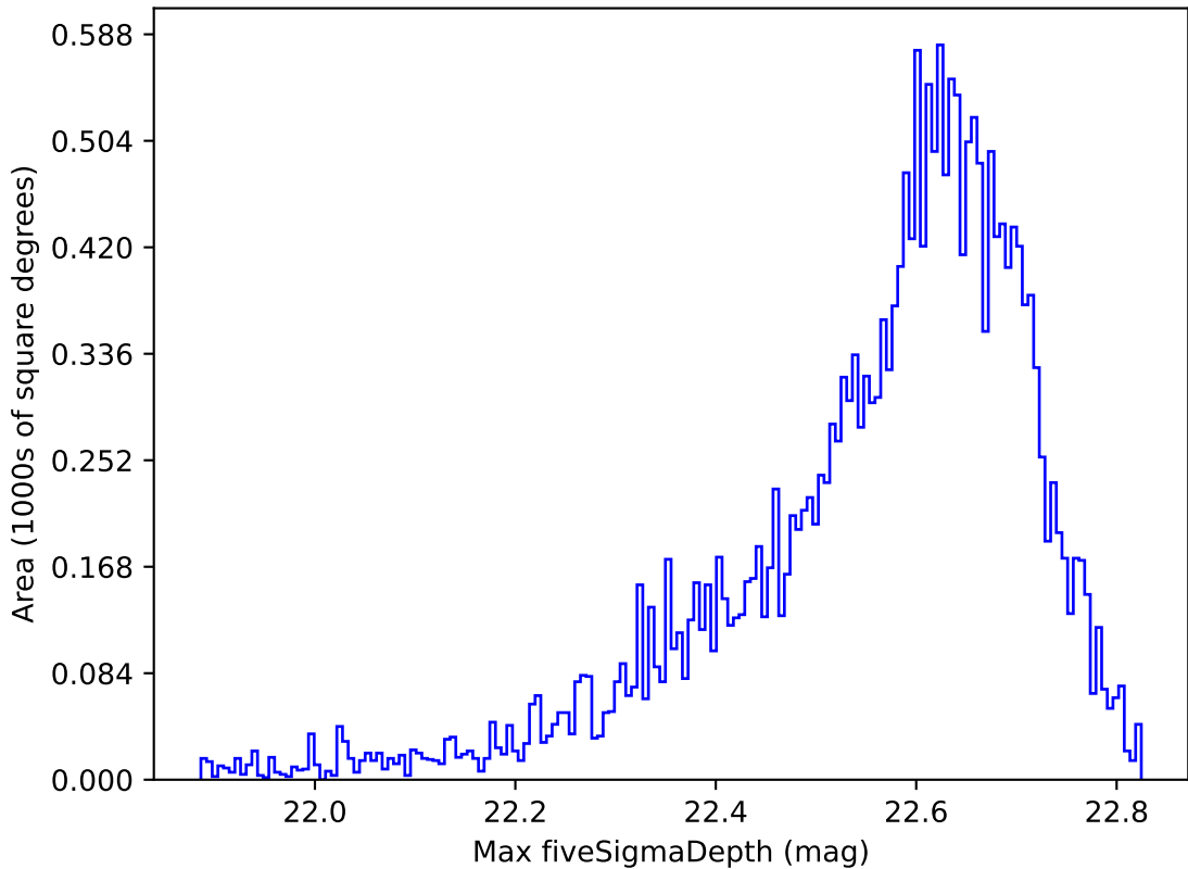
ddf_loaded_half_fl2_v3.4_10yrs All sky y band: Max fiveSigmaDepth
