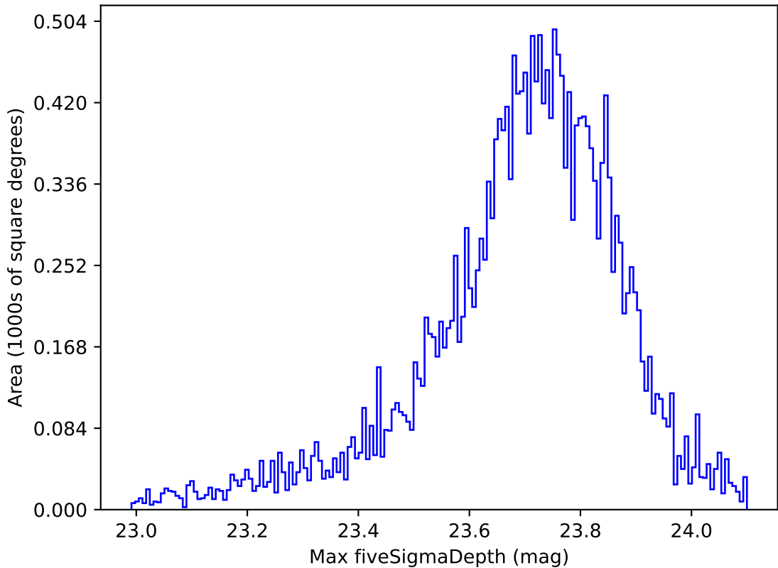
ddf_loaded_half_fl2_v3.4_10yrs All sky u band: Max fiveSigmaDepth
