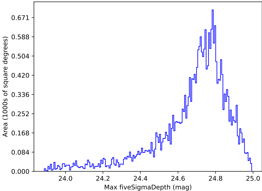
ddf_loaded_half_fl2_v3.4_10yrs All sky r band: Max fiveSigmaDepth
