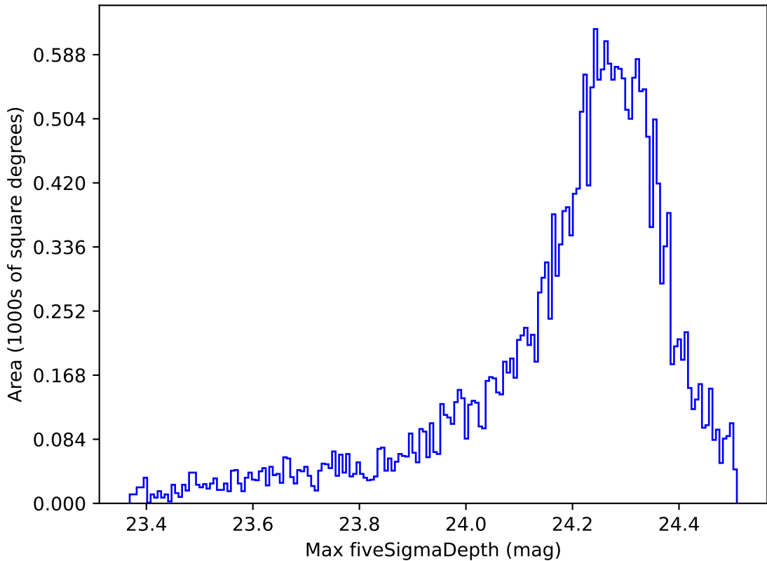
ddf_loaded_half_fl2_v3.4_10yrs All sky i band: Max fiveSigmaDepth
