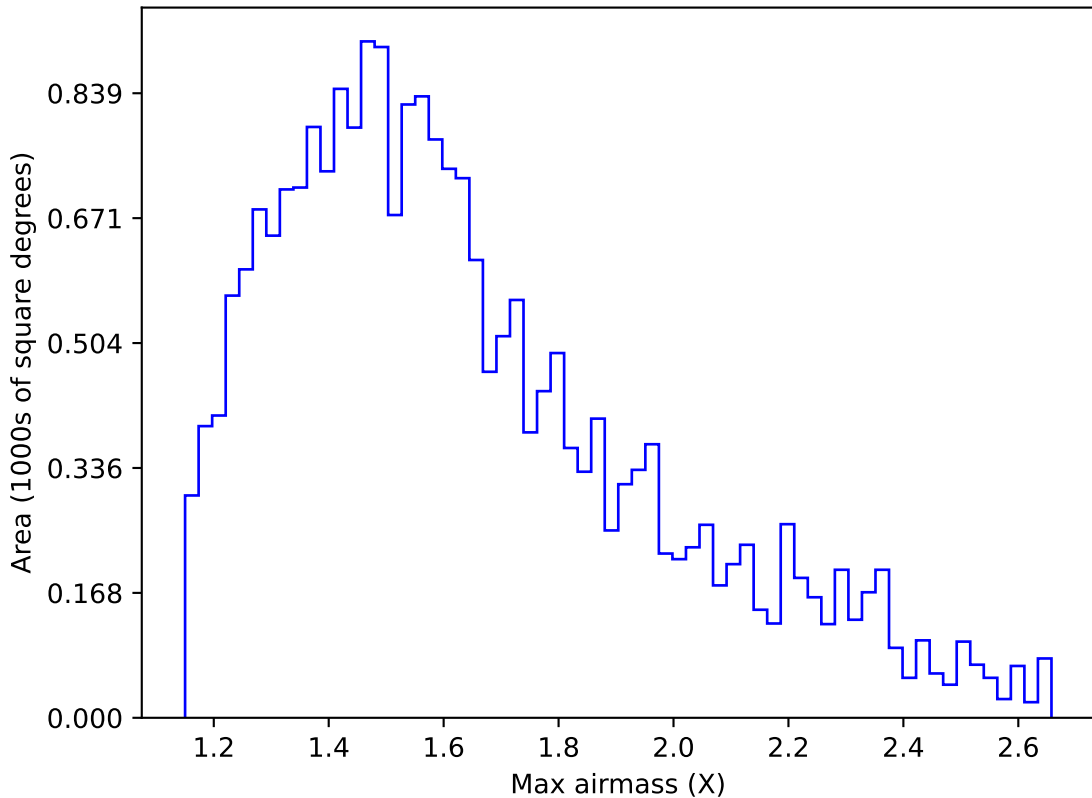
ddf_loaded_half_f12_v3.4_10yrs Yr 1 y band: Max airmass
