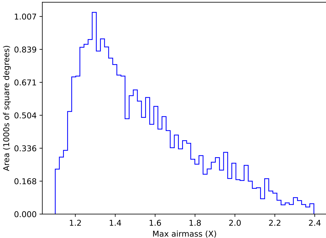
ddf_loaded_half_f12_v3.4_10yrs Yr 1 u band: Max airmass
