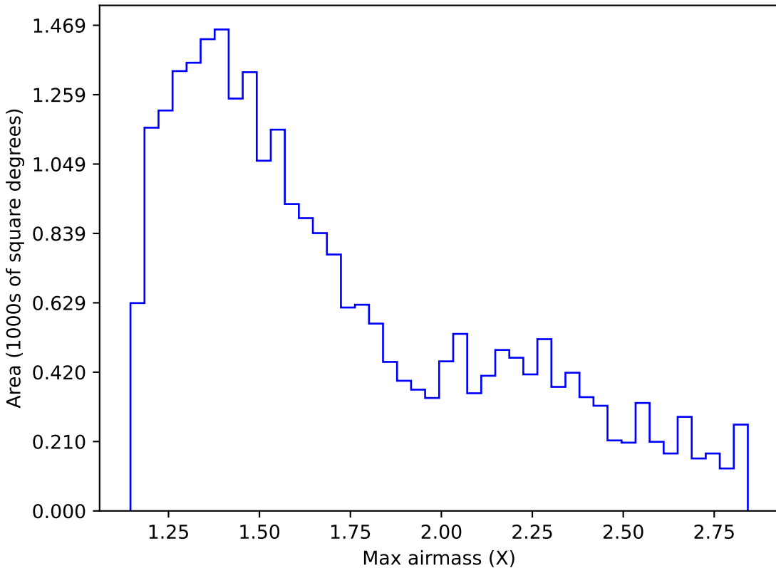
ddf_loaded_half_fl2_v3.4_10yrs Yr 1 i band: Max airmass
