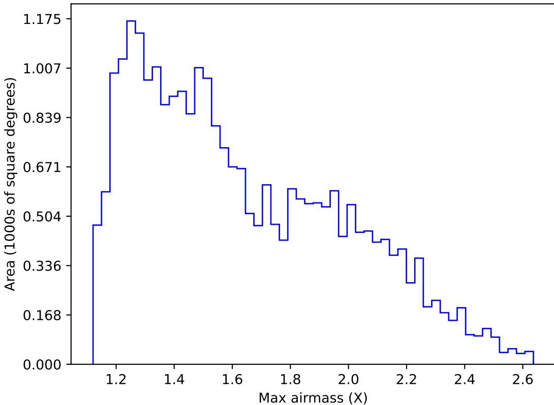
ddf_loaded_half_f12_v3.4_10yrs Yr 1 g band: Max airmass
