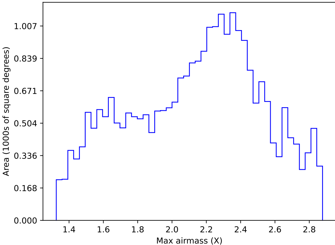
ddf_loaded_half_fl2_v3.4_10yrs Yr 1 all bands: Max airmass
