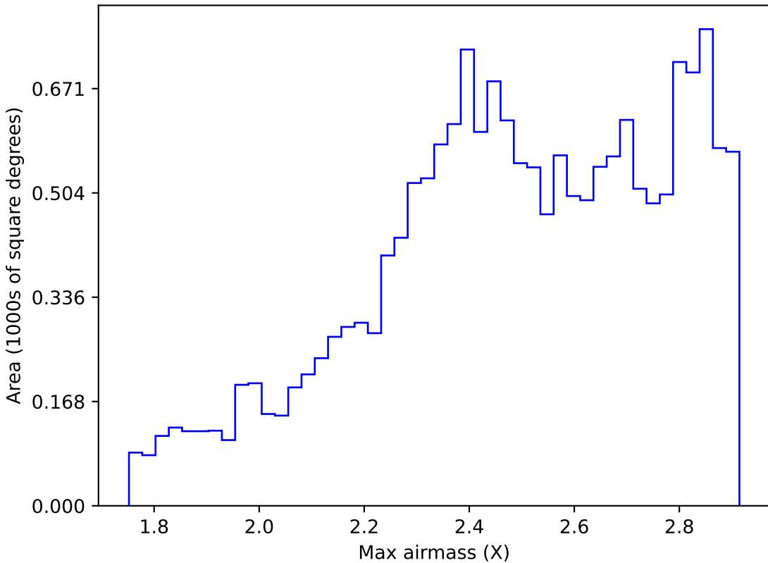
ddf_loaded_half_fl2_v3.4_10yrs WFD z band: Max airmass
