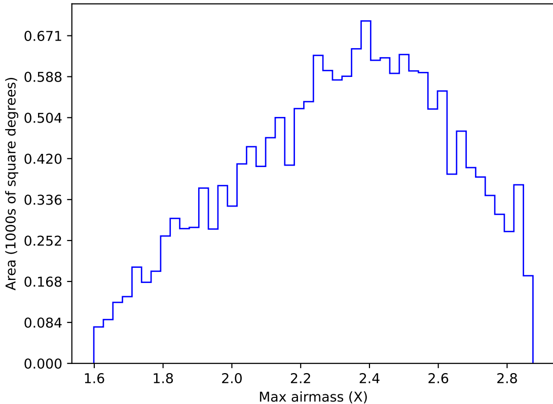
ddf_loaded_half_fl2_v3.4_10yrs WFD y band: Max airmass
