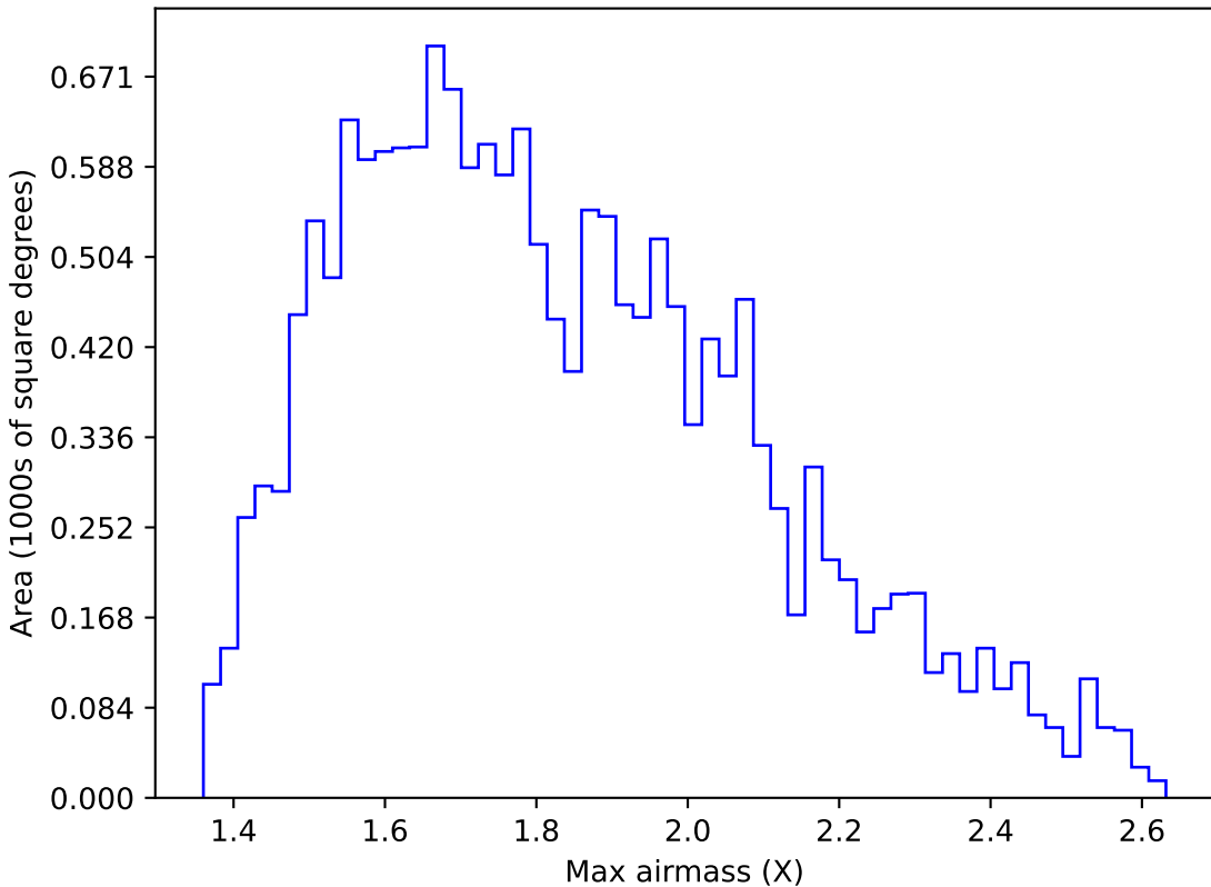
ddf_loaded_half_fl2_v3.4_10yrs WFD u band: Max airmass
