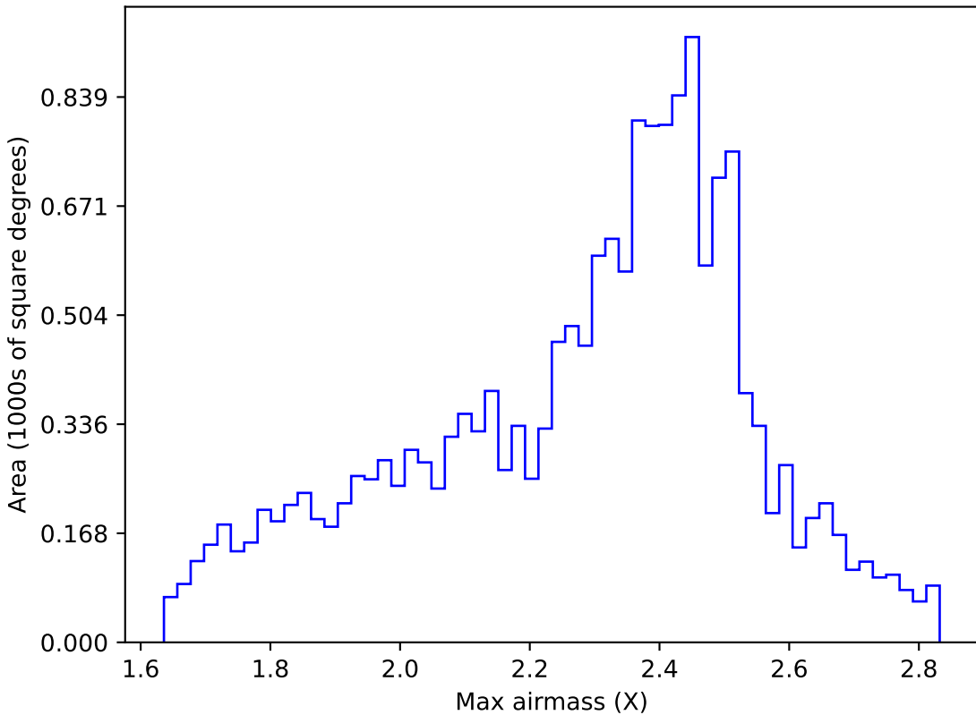
ddf_loaded_half_fl2_v3.4_10yrs WFD r band: Max airmass
