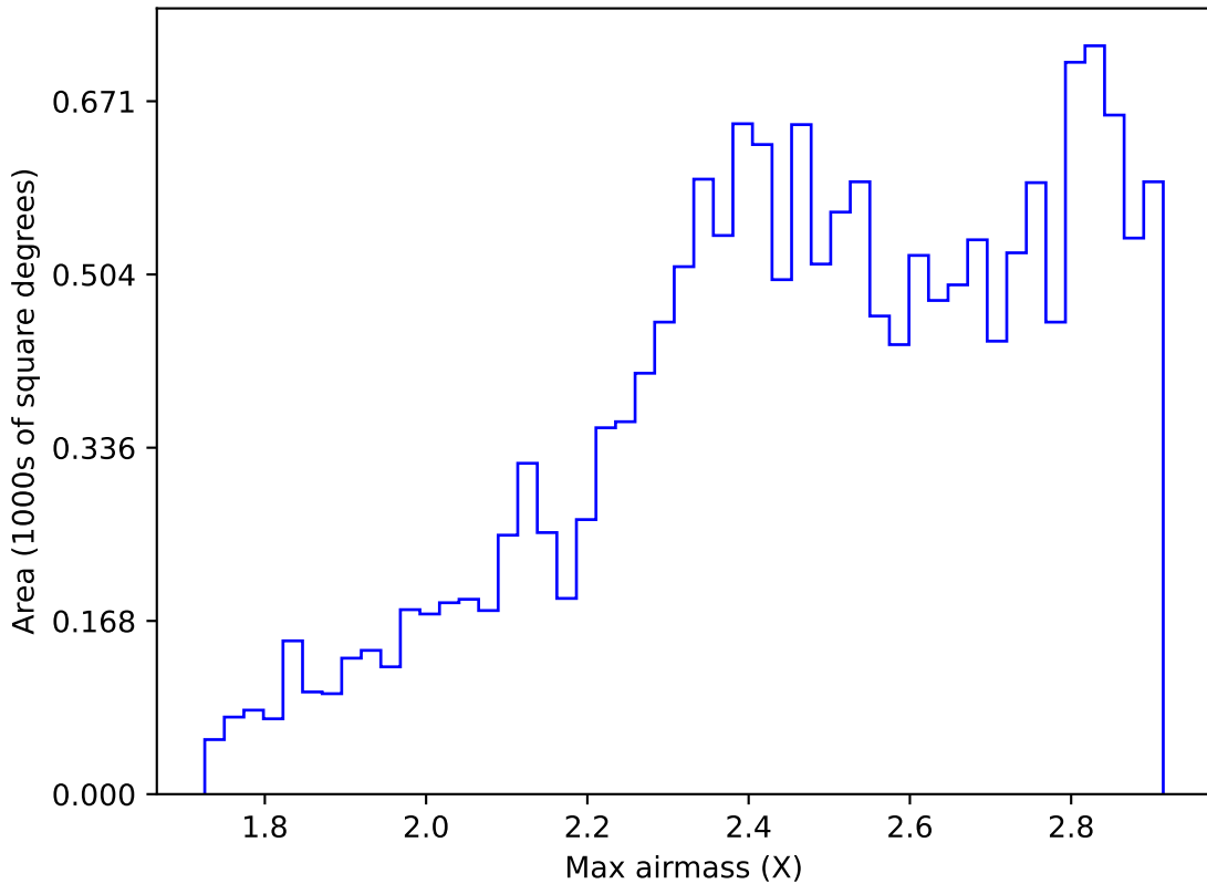
ddf_loaded_half_f12_v3.4_10yrs WFD i band: Max airmass
