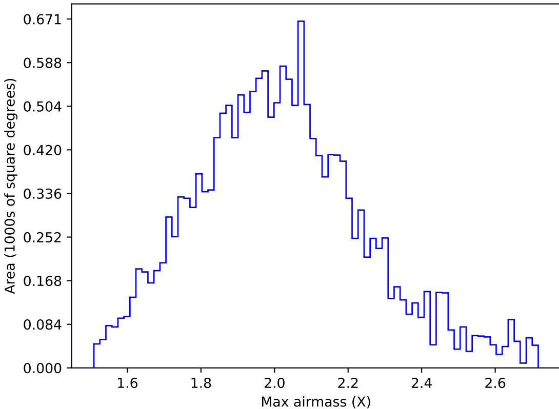
ddf_loaded_half_fl2_v3.4_10yrs WFD g band: Max airmass
