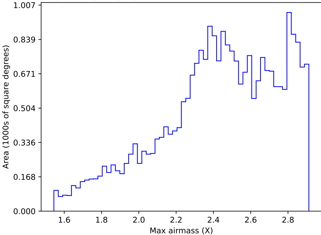
ddf_loaded_half_fl2_v3.4_10yrs All sky z band: Max airmass
