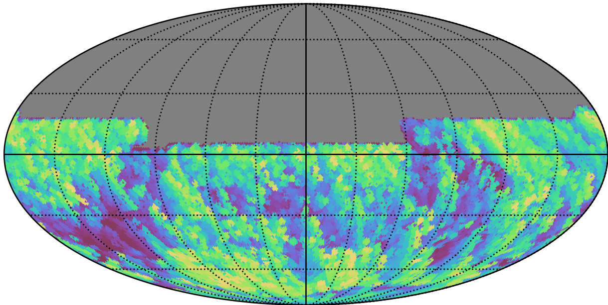
ddf_loaded_half_f12_v3.4_10yrs All sky y band: Max airmass
