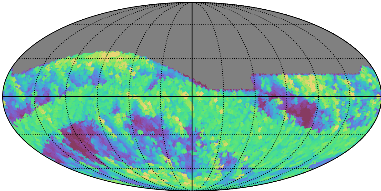
ddf_loaded_half_fl2_v3.4_10yrs All sky r band: Max airmass
