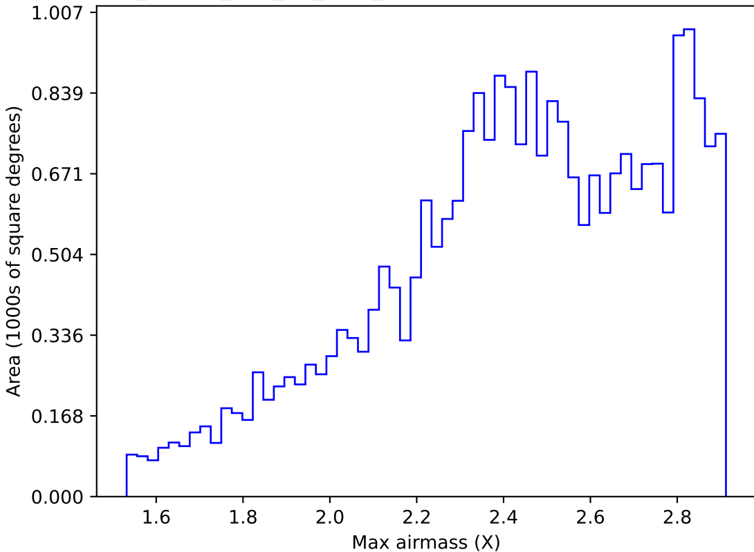
ddf_loaded_half_fl2_v3.4_10yrs All sky i band: Max airmass
