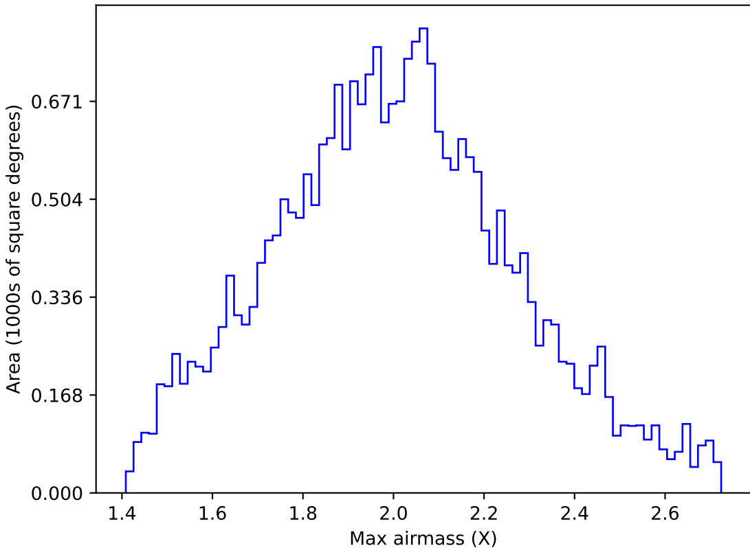
ddf_loaded_half_fl2_v3.4_10yrs All sky g band: Max airmass
