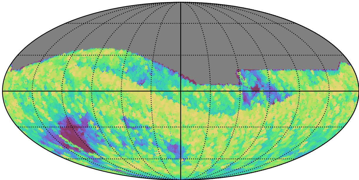
ddf_loaded_half_fl2_v3.4_10yrs All sky all bands: Max airmass
