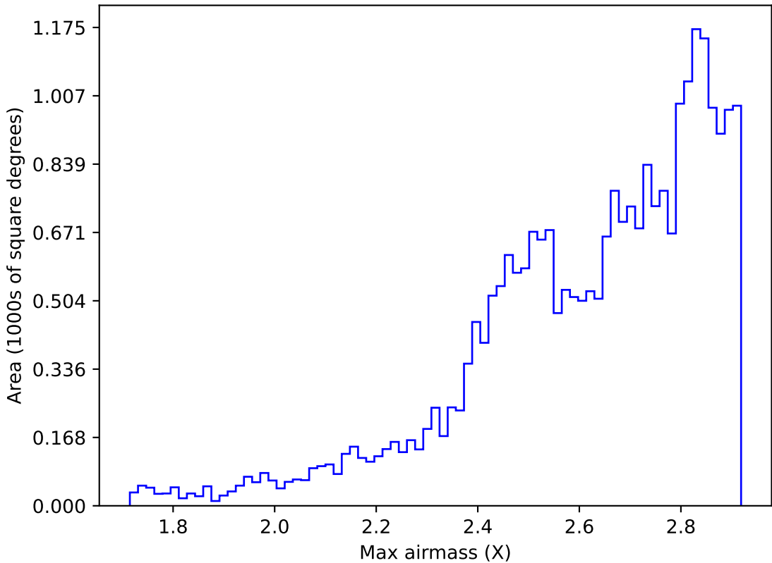
ddf_loaded_half_fl2_v3.4_10yrs All sky all bands: Max airmass
