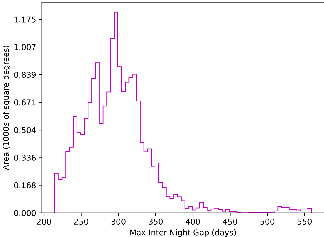
ddf_loaded_half_fl2_v3.4_10yrs WFD z band: Max Inter-Night Gap
