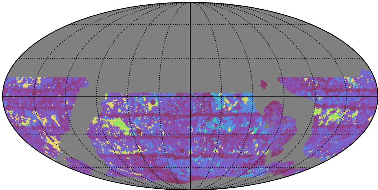
ddf_loaded_half_fl2_v3.4_10yrs WFD y band: Max Inter-Night Gap
